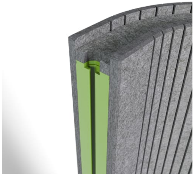
Cooee Spaces Corner – Extrusion Detail
